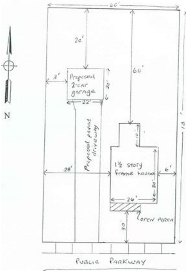
Sample Site Plan
